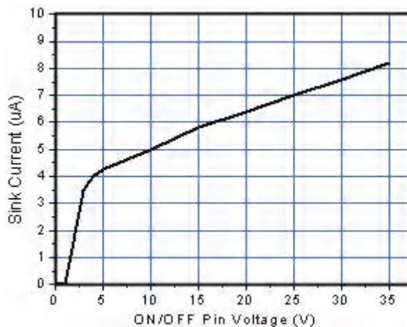
Figure 6. ON/OFF Pin Sink Current
