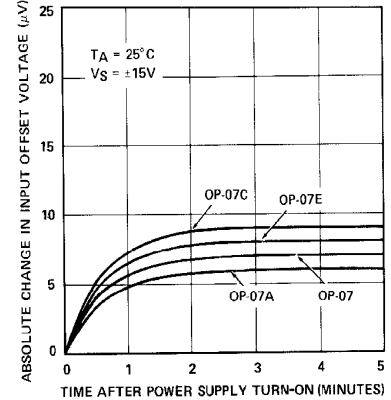
WARM-UP DRIFT
