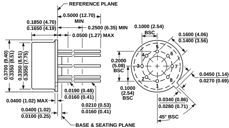
8-Pin Metal Header [TO-99]
