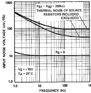
TOTAL INPUT NOISE VOLTAGE vs FREQUENCY
