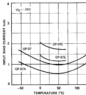
INPUT BIAS CURRENT vs TEMPERATURE
