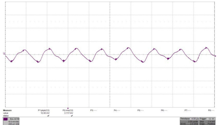
Fig. 36: Input reflected ripple current, i_c (500 mA/div.), measured at input terminals at full rated load current. Refer to Fig. 2 for test setup. RMS input ripple current i_c = 3.12 \times 0.5A = 1.56A_{RMS} .
