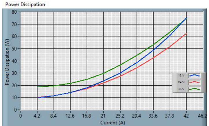
Fig. 8: 24S24.42FXP (ROHS) Power Dissipation
