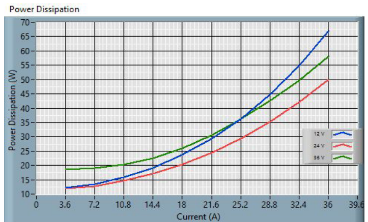
Fig. 10: 24S28.36FXP (ROHS) Power Dissipation
