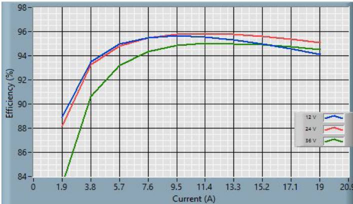
Fig. 13: 24S53.19FXP (ROHS) Efficiency Curve
