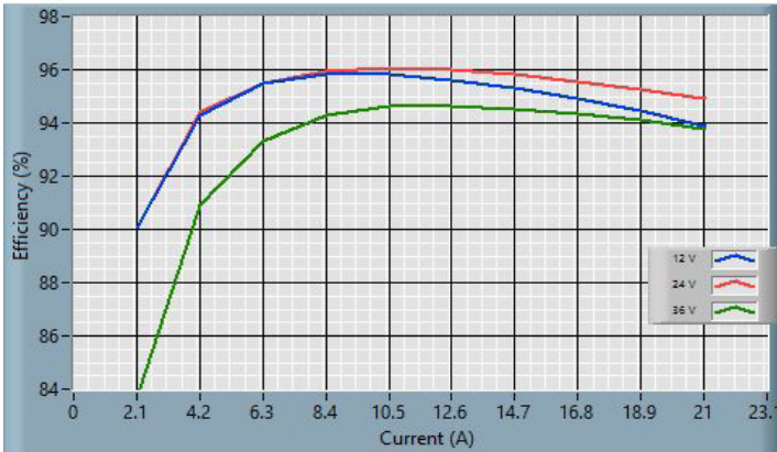
Fig. 11: 24S48.21FXP (ROHS) Efficiency Curve
