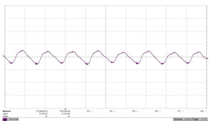
Fig. 24: Input reflected ripple current, i_c (500mA/mV), measured at input terminals at full rated load current. RMS input ripple current i_c = 3.14 \times 0.5A = 1.07 A_{RMS} . (See Fig. 5).
