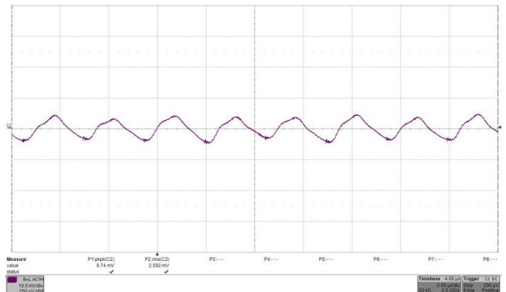
Fig. 30: Input reflected ripple current, i_c , measured at input terminals at full rated load current. Refer to Fig. 2 for test setup. RMS input ripple current i_c = 2.6 \times 0.5A = 1.3A_{RMS} .
