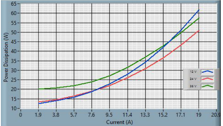
Fig. 14: 24S53.19FXP (ROHS) Power Dissipation
