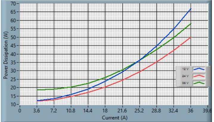
Fig. 12: 24S48.21FXP (ROHS) Power Dissipation
