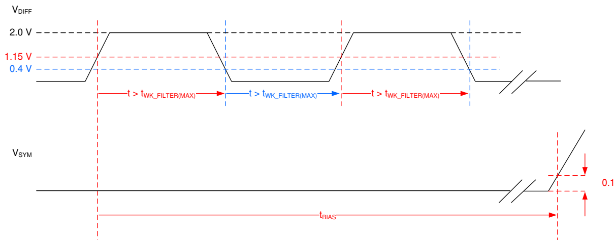
Figure 7-9. Bias Reaction Time Measurement
