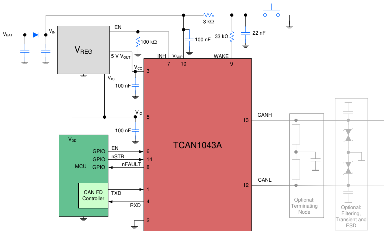
Figure 9-1. Typical Application
