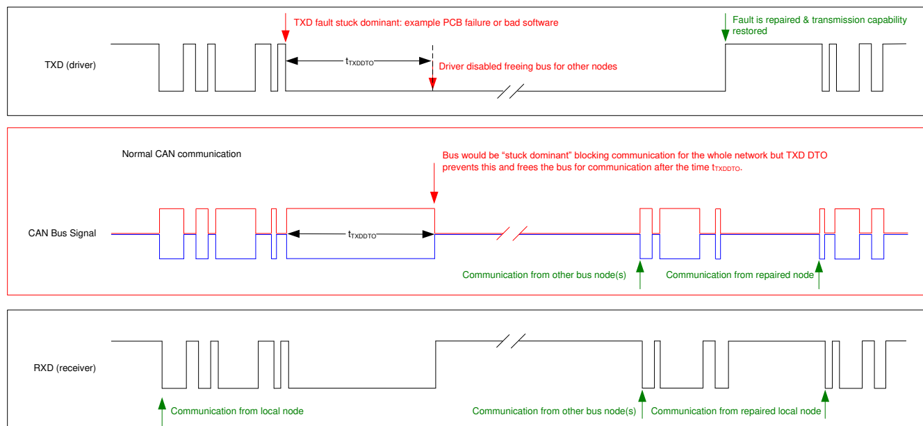
Figure 8-3. Timing Diagram for TXD DTO
