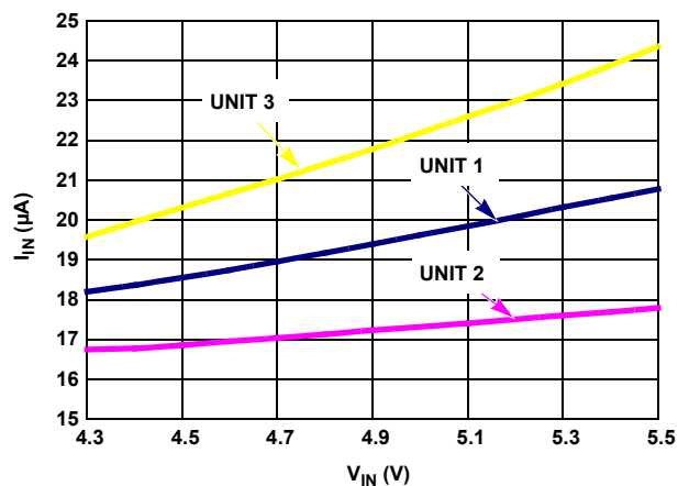
FIGURE 18. I_{IN} vs V_{IN} , 3 TEMPERATURES
