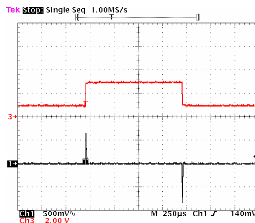
FIGURE 58. LOAD TRANSIENT RESPONSE, 1nF LOAD CAPACITANCE
