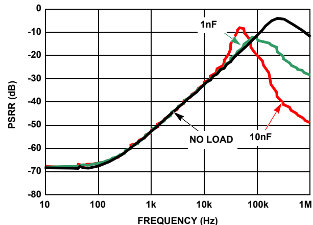
FIGURE 24. PSRR AT DIFFERENT CAPACITIVE LOADS
