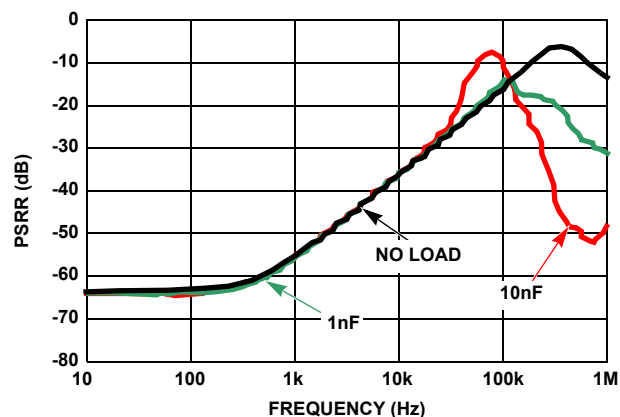
FIGURE 8. PSRR AT DIFFERENT CAPACITIVE LOADS
