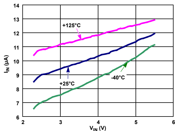
FIGURE 48. I_{IN} vs V_{IN} , 3 TEMPERATURES
