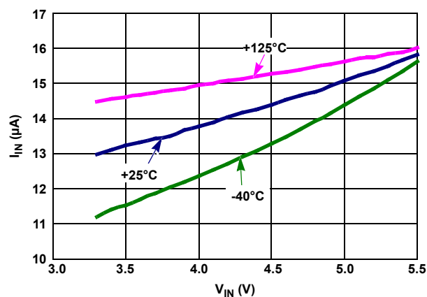
FIGURE 2. I_{IN} vs V_{IN} , 3 TEMPERATURES
