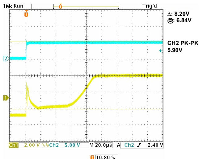
FIGURE 27. TURN-ON TIME, 1kΩ
