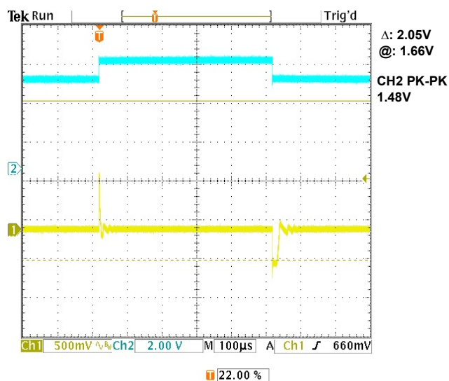
FIGURE 30. LINE TRANSIENT RESPONSE, 1nF LOAD
