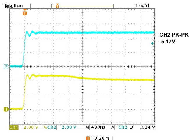
FIGURE 26. TURN-ON TIME, NO LOAD
