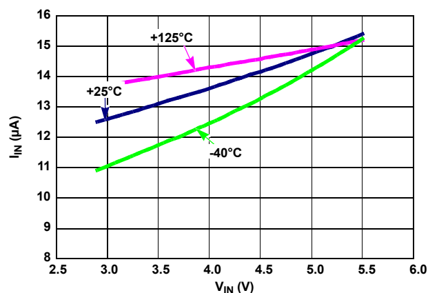
FIGURE 34. I_{IN} vs V_{IN} , 3 TEMPERATURES
