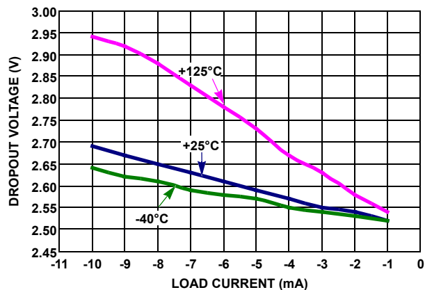
FIGURE 39. LOAD CURRENT vs DROPOUT
