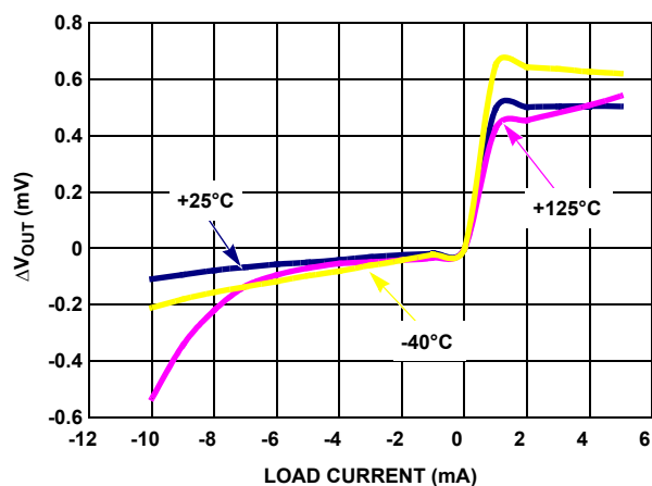
FIGURE 21. LOAD REGULATION
