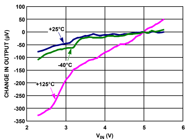
FIGURE 52. LINE REGULATION OVER-TEMPERATURE
