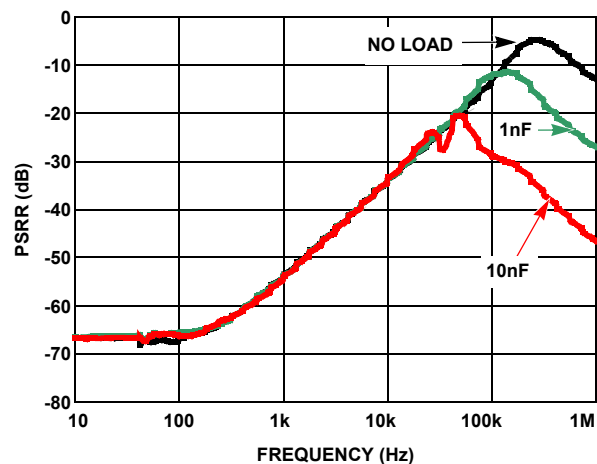
FIGURE 54. PSRR AT DIFFERENT CAPACITIVE LOADS
