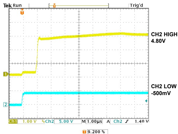
FIGURE 10. TURN-ON TIME, NO LOAD
