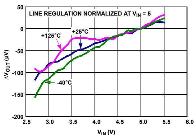
FIGURE 38. LINE REGULATION OVER-TEMPERATURE
