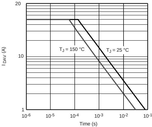
Single Pulse Avalanche Current Capacity vs. Time
