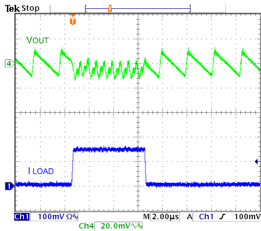
Figure 24. 1.82V OUT Load Transient, 10-160mA, t_R/t_F=100ns with Optional 2.2μF C OUT
