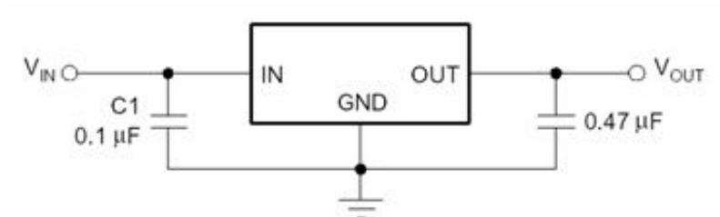
Figure 3. Application circuit, fixed version
