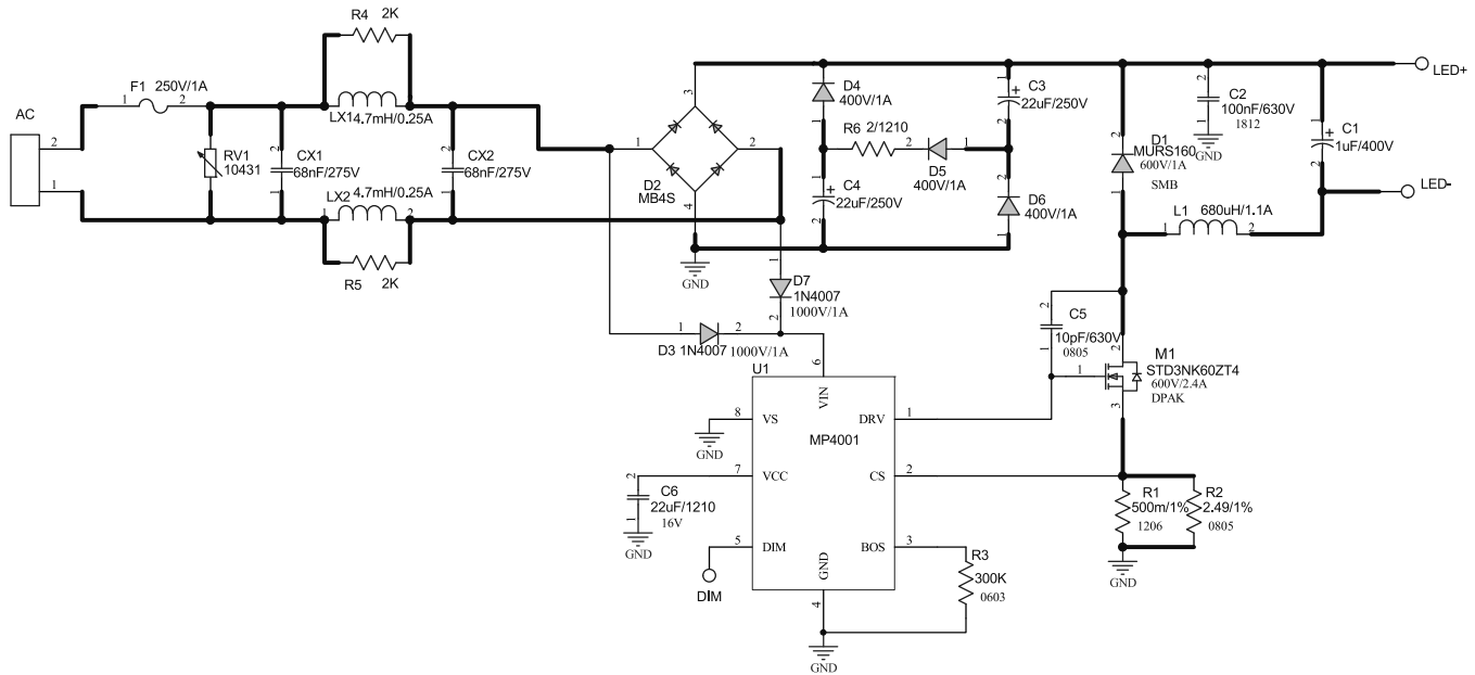
Figure 6: Schematic
