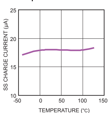
SS Charge Current vs. Temperature
