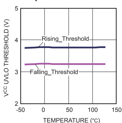
V_{CC} UVLO Threshold vs. Temperature
