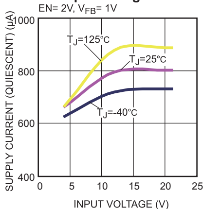
Supply Current (Quiescent) vs. Input Voltage EN= 2V, V_{FB} = 1V
