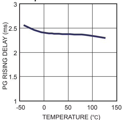
PG Rising Delay vs. Temperature
