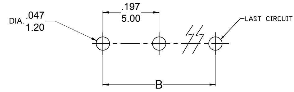
Reference PCB Hole
