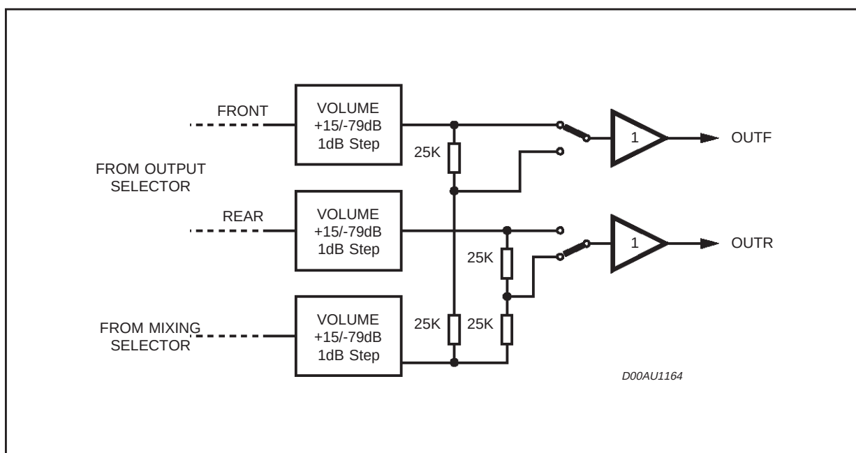
Figure 21. Output Selector
