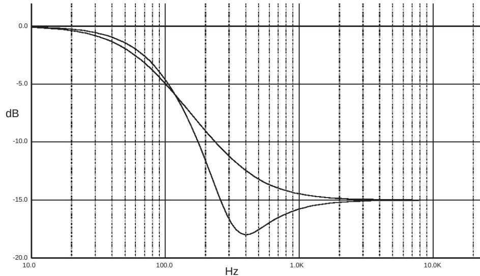
Figure 4. 1st and 2nd Order Loudness @ Attn. = 15dB, f_c=400\text{Hz}
