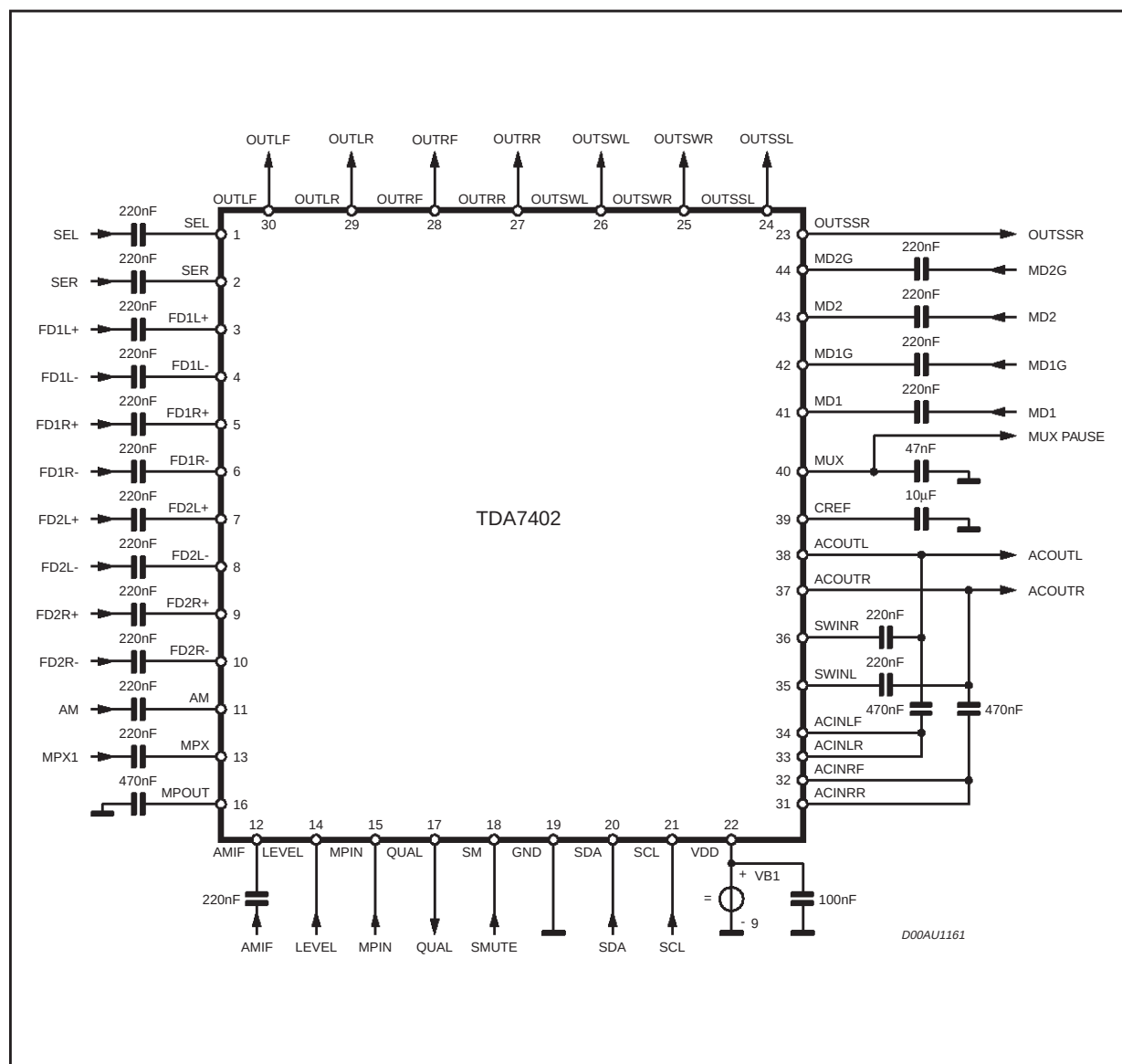
Figure 34. Application Diagram (standard configuration)
