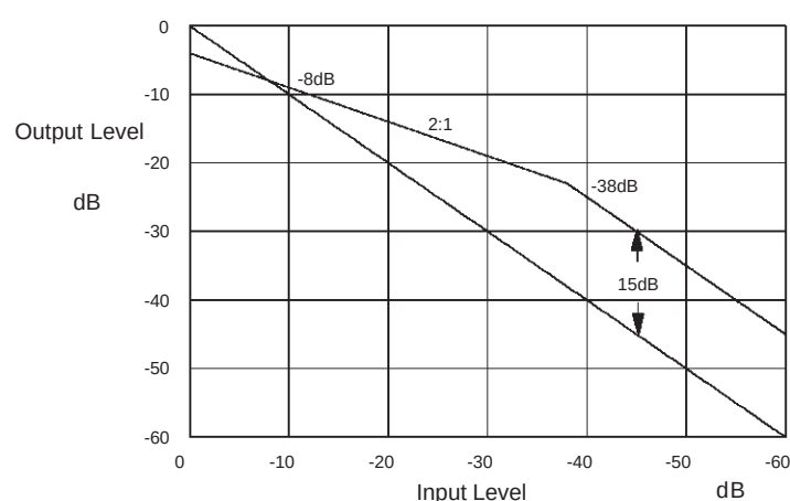
Figure 16. Compander Characteristic
