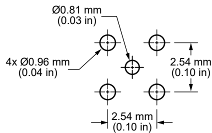
Figure 2. Recommended PCB Dimensions for the CONSMP001-1
