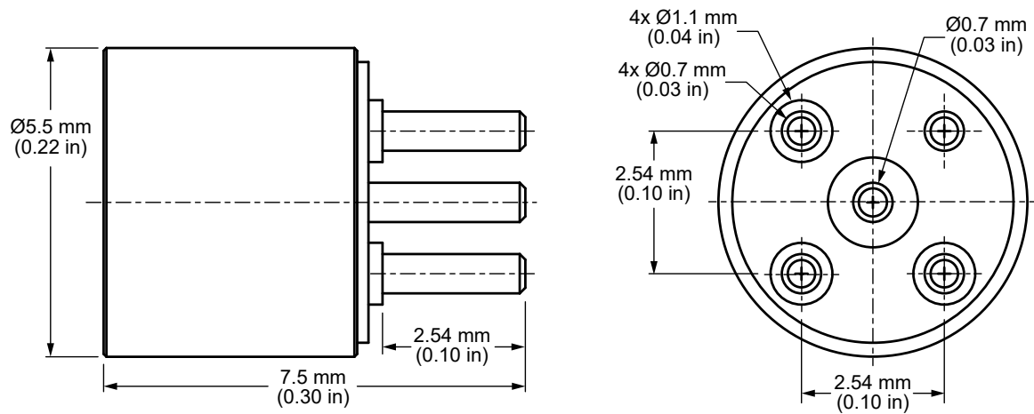
Figure 1. Product Dimensions for the CONSMP001-1 Connector Table
