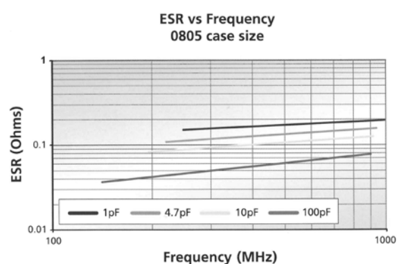
Typical performance data - 0805 chip size*
