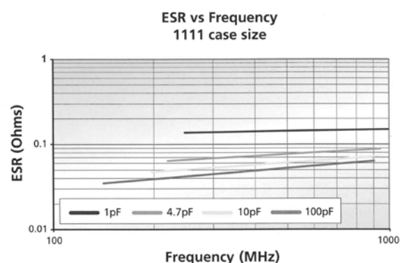
Typical performance data - 1111 chip size*
