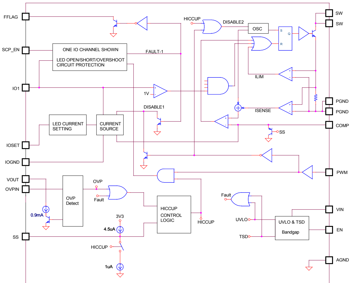
Figure 1. SC445 Block Diagram
