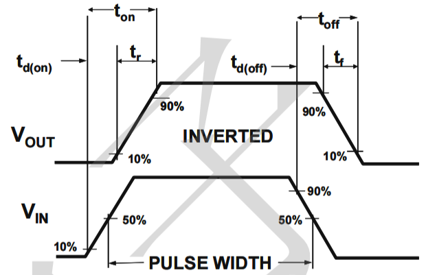
Figure 2: Switching Waveforms
