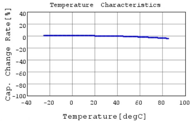
GRM022B11A101KA01 C-Temp. capchange, DC0.0V,
