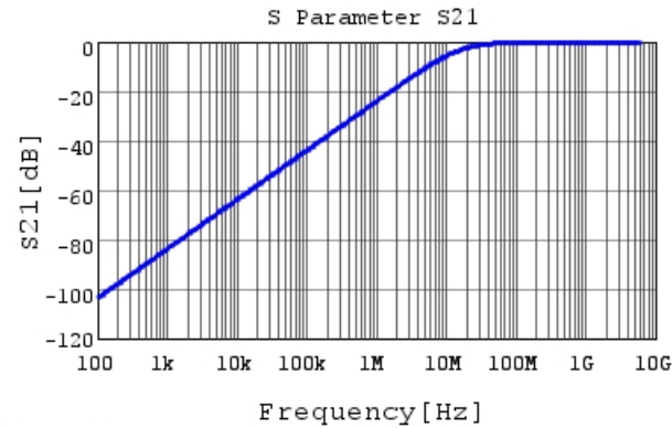
GRM022B11A101KA01 S21 DC0V,20degC
