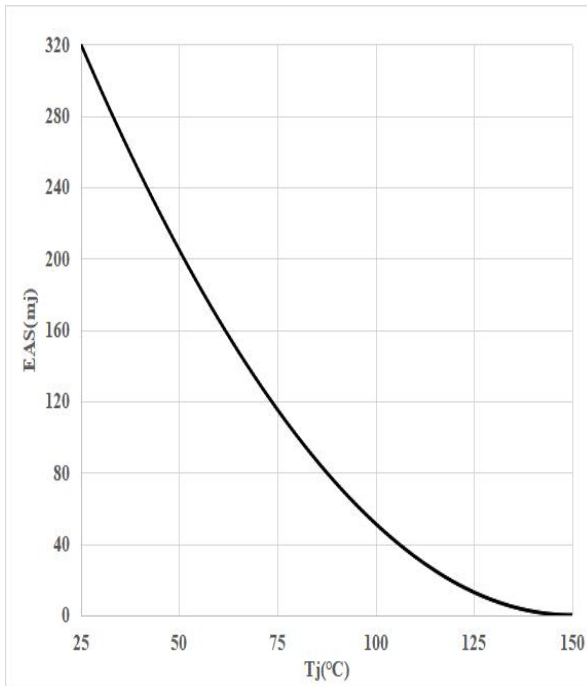
Figure 15: Avalanche Energy
