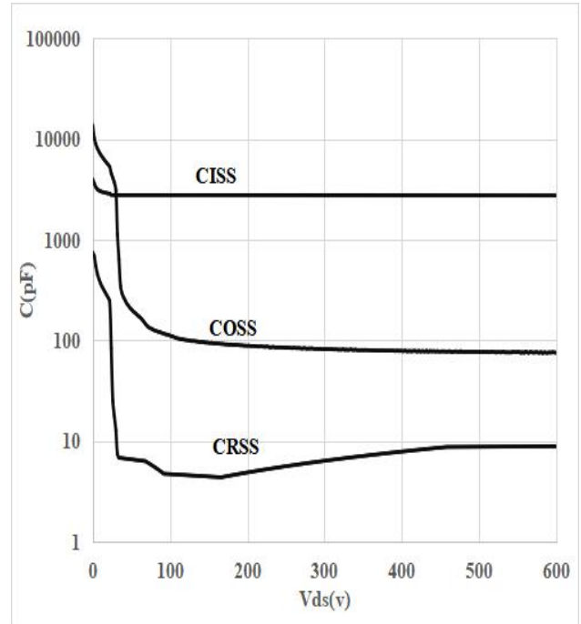
Figure 16: Typ. Capacitances
