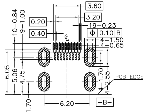
RECOMMENDED PCB LAYOUT(.XX±0.05) CONNECTOR SIDE(TOP VIEW)
