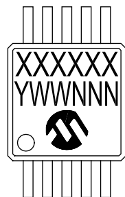
10-Lead MSOP (3x3 mm)
