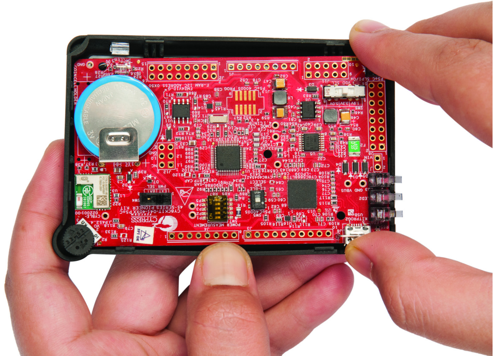
Figure 3-8. Pull out the main board from the case
