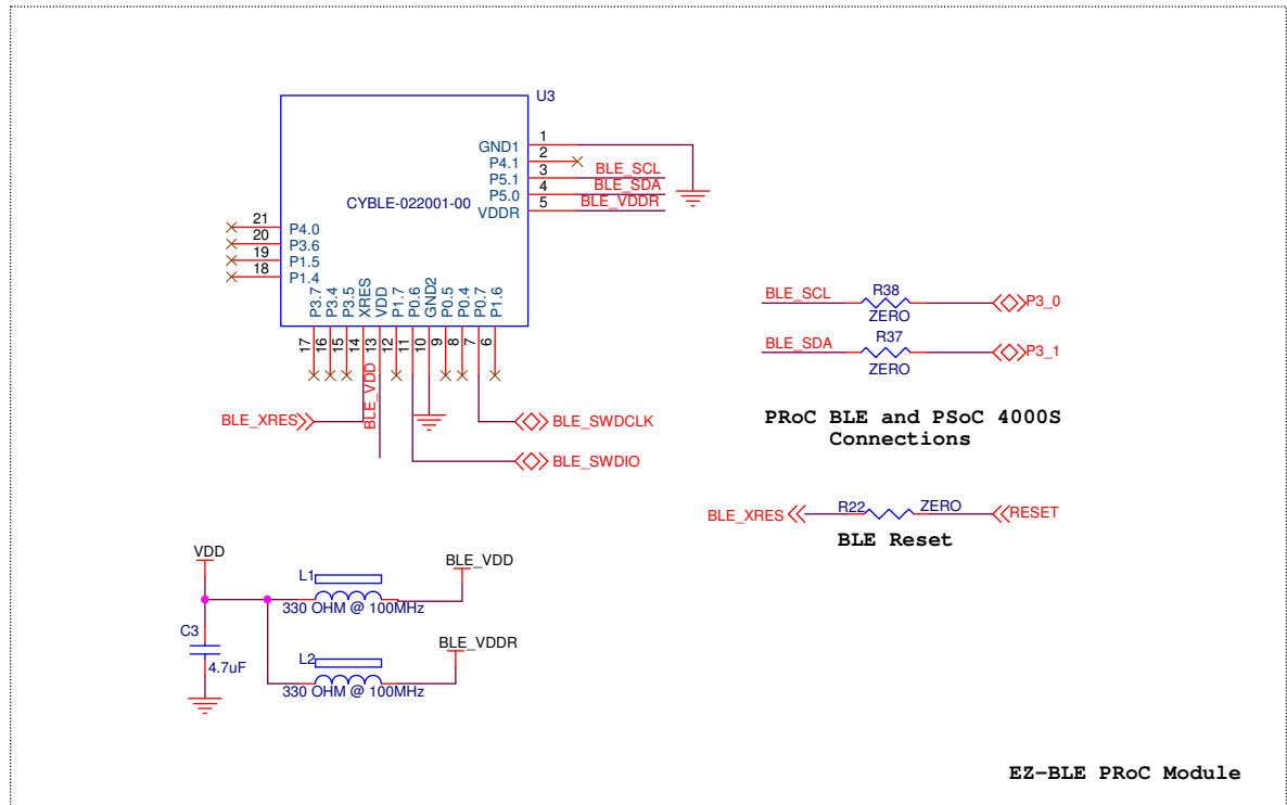
Figure A-13. EZ-BLE PSoC Connections
