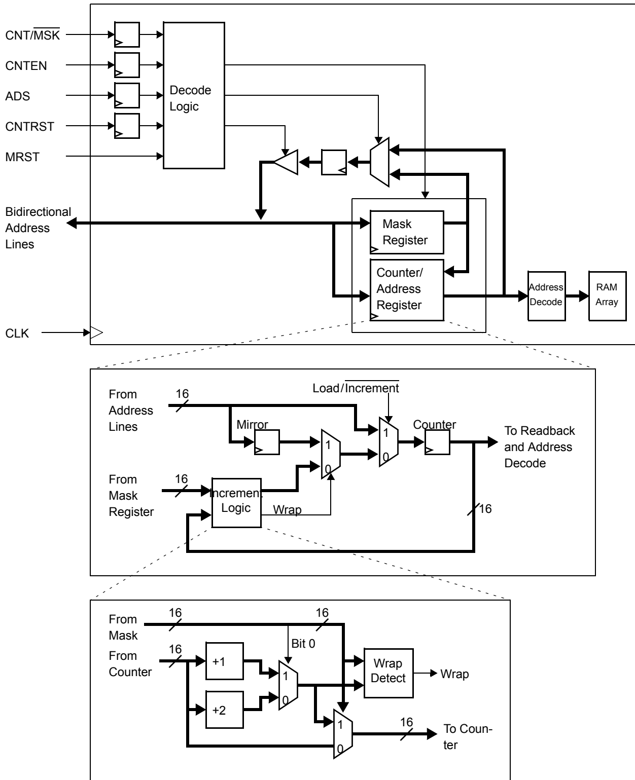
Figure 3. Counter, Mask, and Mirror Logic Block Diagram
