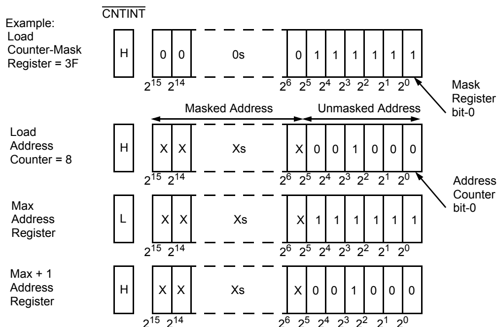
Figure 2. Programmable Counter-Mask Register Operation [17]
