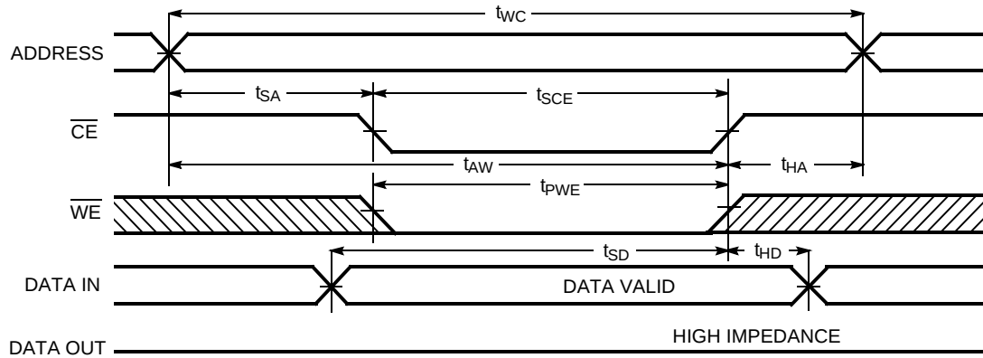
Figure 6. Write Cycle No. 2 ( \overline{\text{CE}} Controlled) [13, 14]
