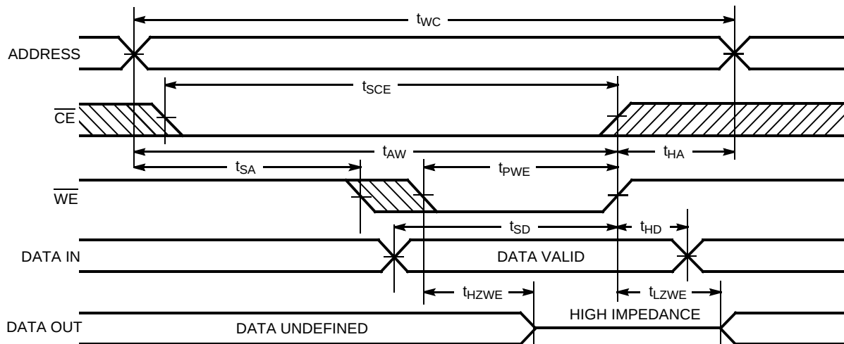
Figure 5. Write Cycle No. 1 (WE Controlled) [12]
