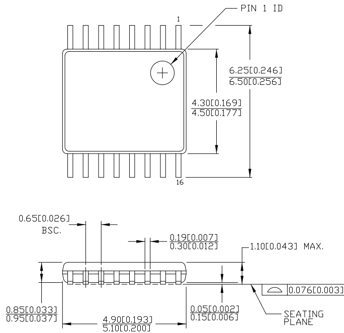
Figure 8. 16-pin TSSOP 4.40 mm Body ZZ16
