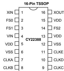
Figure 1. 16-pin TSSOP pinout
