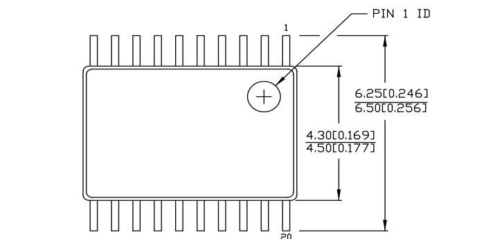
Figure 11. 20-pin TSSOP (4.40 mm Body) Z20.173/ZZ20.173 Package Outline, 51-85118
