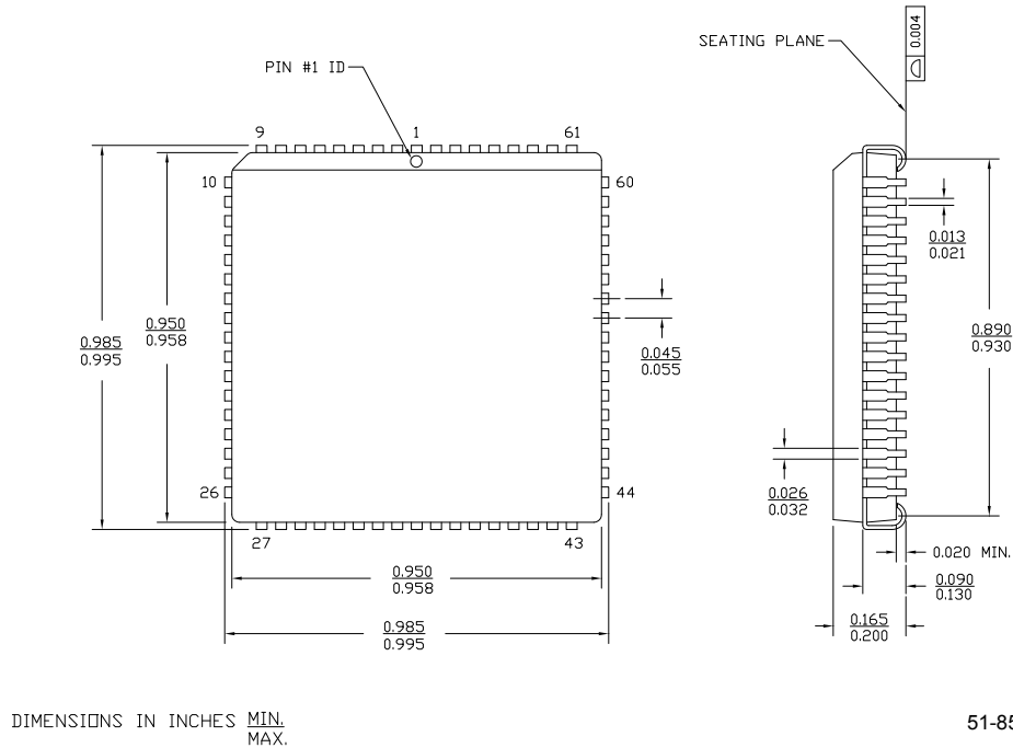
Figure 20. 68-Pin Plastic Leaded Chip Carrier, 51-85005
