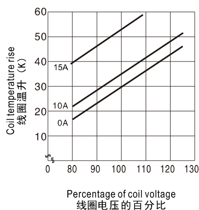
Coil temperature rise 线圈温升
