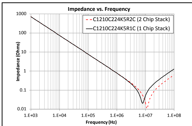
Impedance – 1210, .22 \mu F, 50 V X7R
