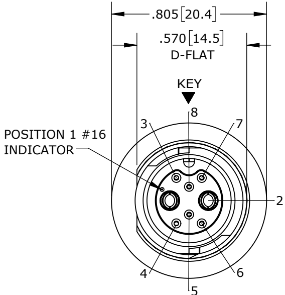
MATING FACE W7A82-8SG-P-300 SHOWN
