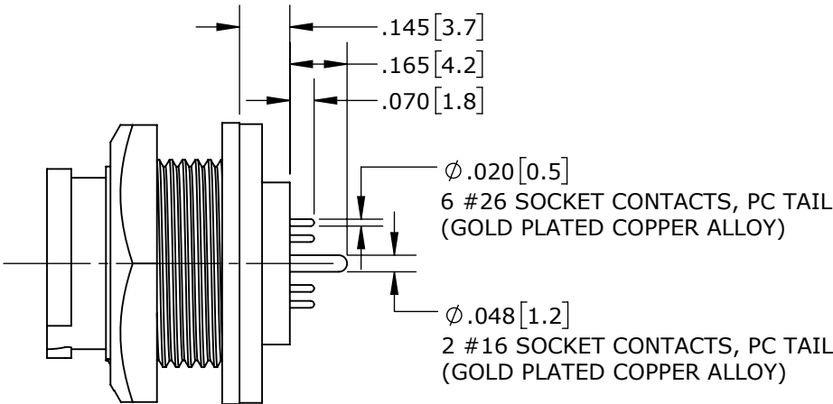
PC TAIL CONTACTS W7A81-8SG-P-3ES SHOWN
