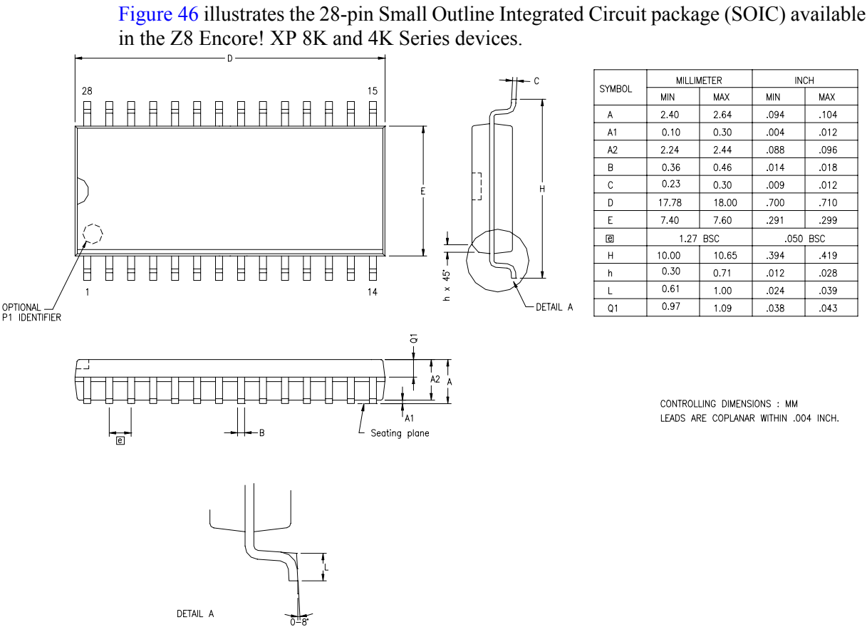
Figure 46. 28-Pin Small Outline Integrated Circuit Package (SOIC)
