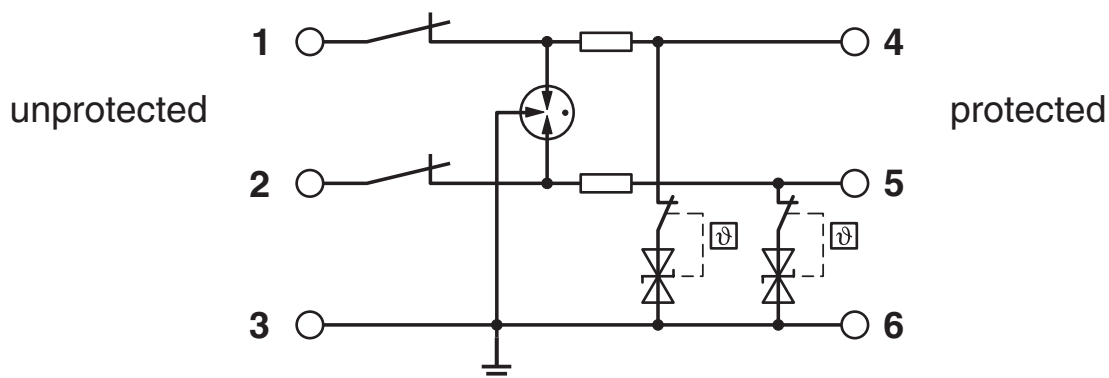
Circuit diagram
