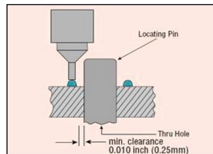
Figure 7-9 Dispensing path obstructed
