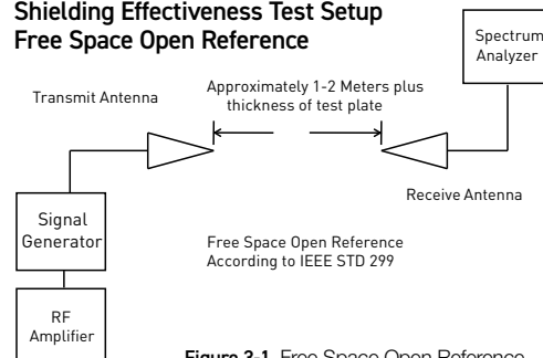
Figure 3-1. Free Space Open Reference
