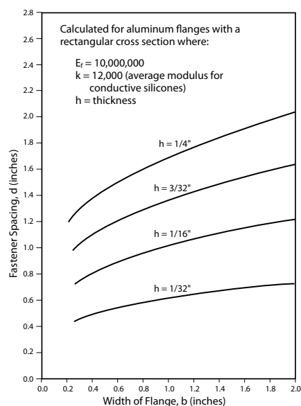
Figure 1-13. Fastener Spacing
