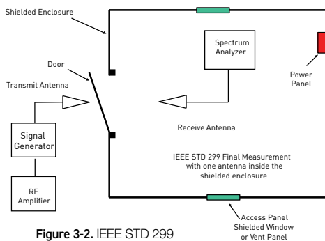
Figure 3-2. IEEE STD 299
