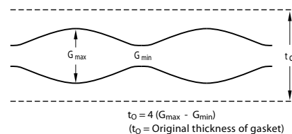
Figure 1-10: Gasket Deflection Along a Flange
