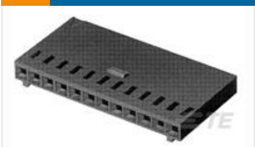
TE Part #102241-1 03 MODIV HSG COMP SR .100 POL
