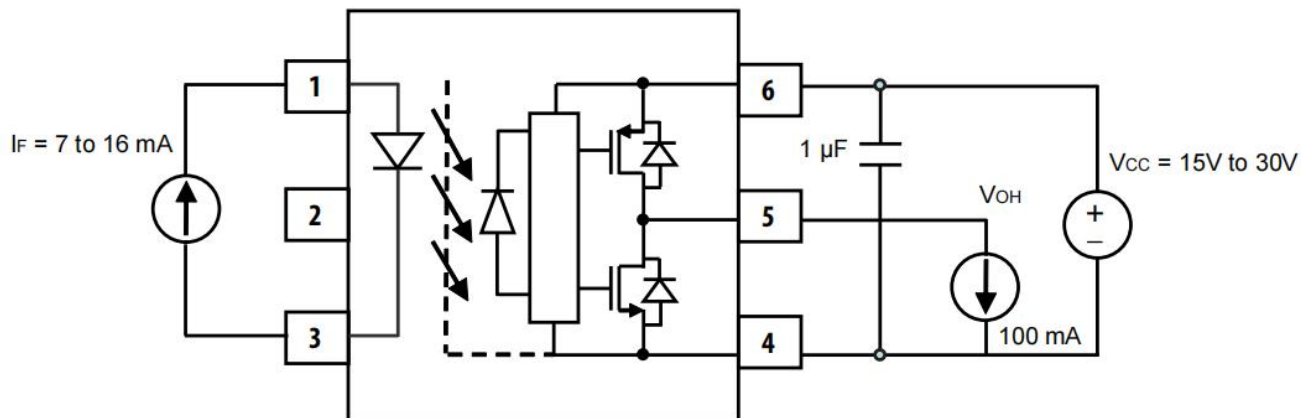
Fig.16 V_{OH} Test Circuit
