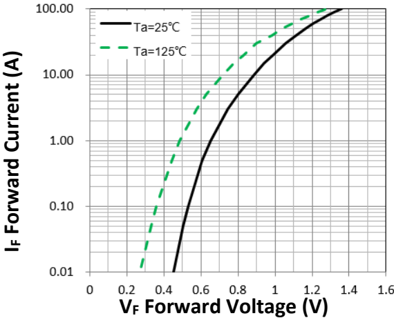
Figure 1. Forward Characteristic(typ.)
