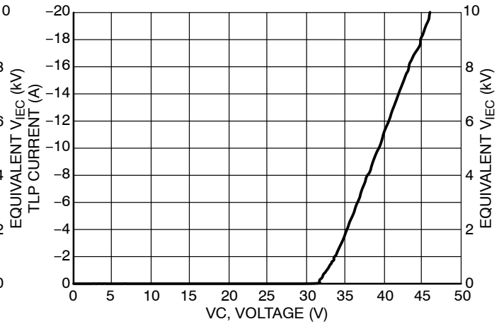
Figure 10. Negative TLP I-V Curve
