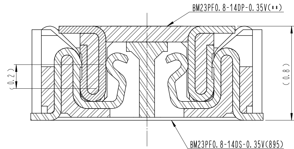
ENGAGEMENT FIGURE (50:1)
