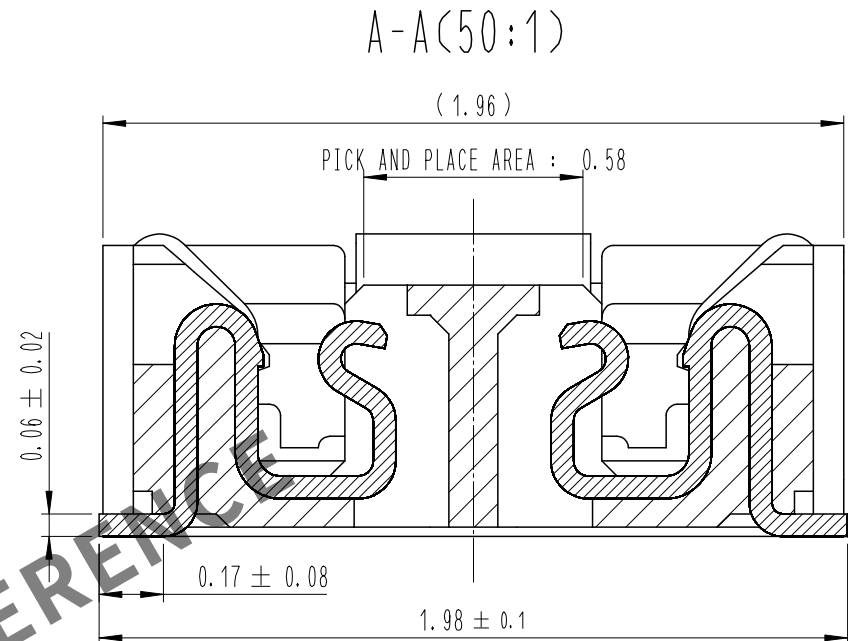
ENGAGEMENT FIGURE (50:1)
