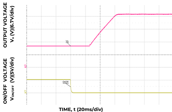
Figure 17. Typical Start-up Using On/Off Voltage (I o = I o, max )
