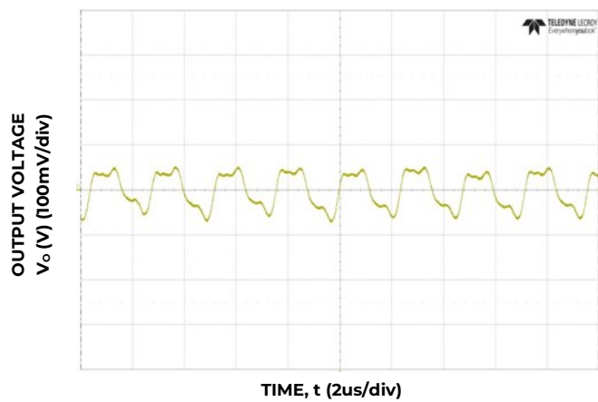
Figure 9. Typical output ripple (C o =66μF ceramic, V IN = 12V, I o = I o, max )
