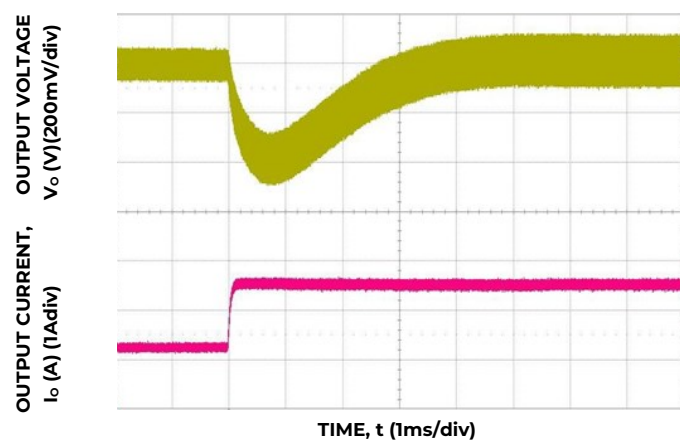
Figure 10. Transient Response to Dynamic Load Change from 50 % to 100% at 12V IN , C OUT = 3x10μF+220μF, C Tune =3300pF, R Tune =30.1kΩ
