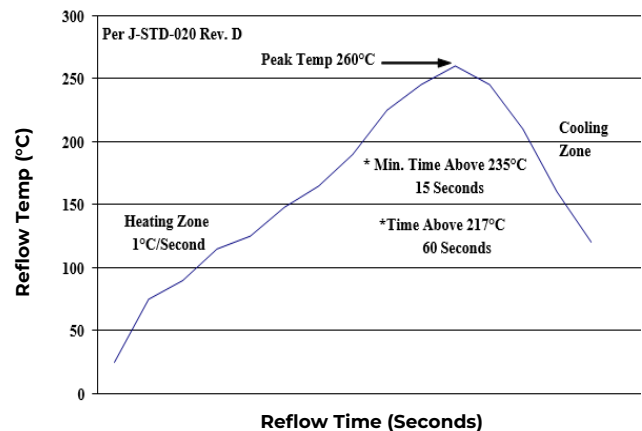
Figure 35. Recommended linear reflow profile using Sn/Ag/Cu solder.
