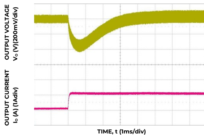
Figure 16. Transient Response to Dynamic Load Change from 50% to 100% at 12V in , C OUT = 9x10uF, C Tune =3300pF, R Tune =30.1Ω
