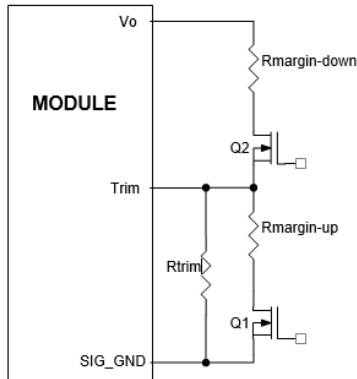
Figure 30 Circuit Configuration for margining Output voltage.
