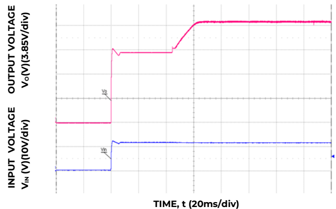
Figure 6. Typical Start-up Using Input Voltage (V IN = 12V, I o = I o, max )
