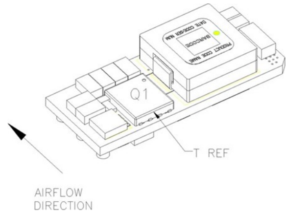
Figure 33. Preferred airflow direction and location of hot-spot of the module ( T_{ref} ).
