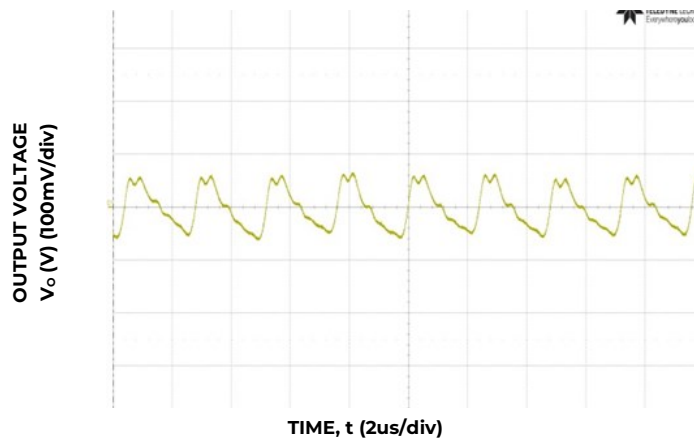
Figure 21. Typical output ripple and noise ( C_o=66\mu\text{F} ceramic, V_{IN} = 12V , I_o = I_{o, \max} )
