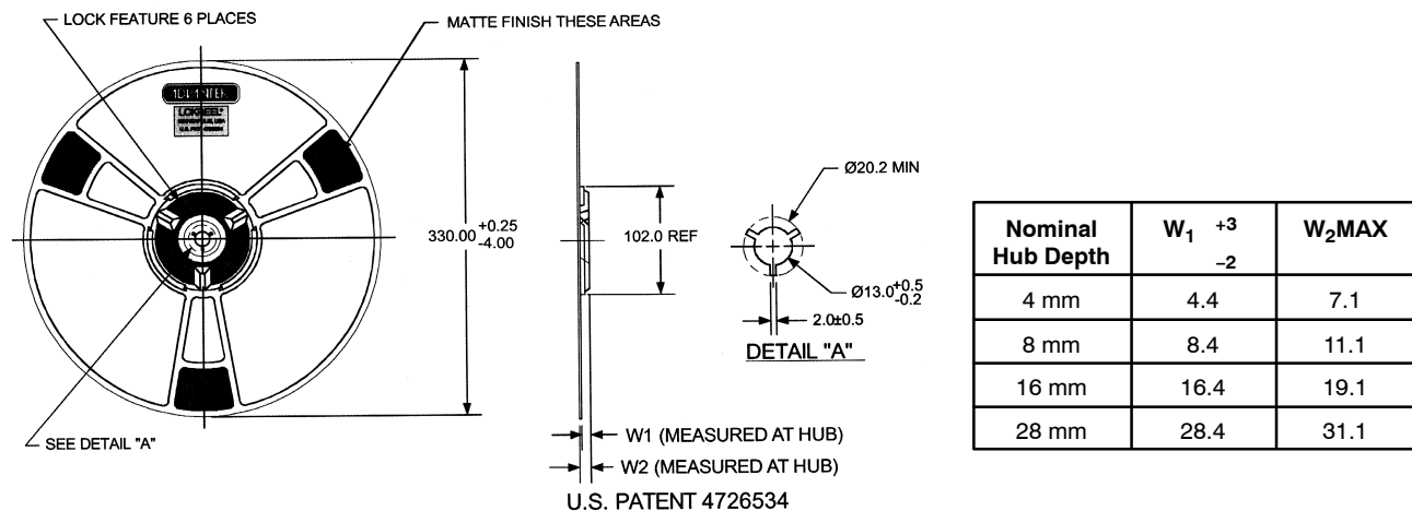
Figure 13. Reel Dimensions
