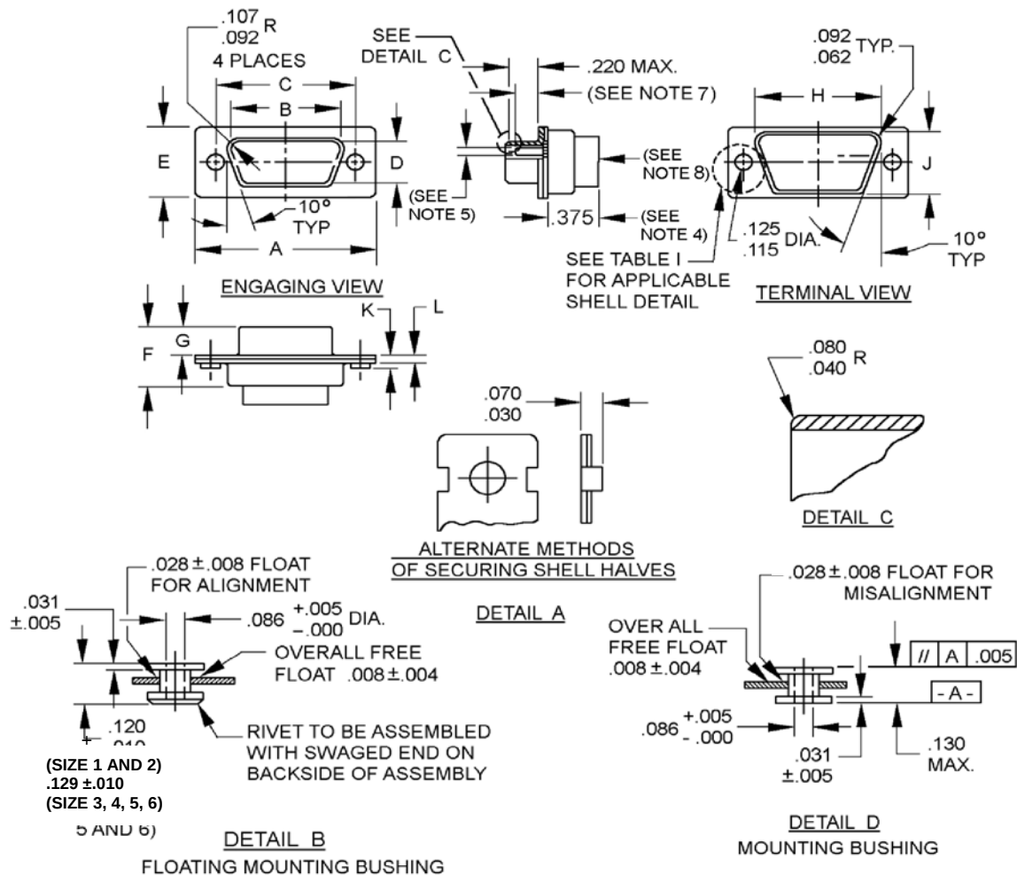
FIGURE 1. Shell, plug, crimp type.
