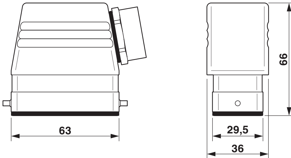
Dimensional drawing
