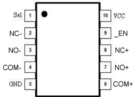
MSOP-10
