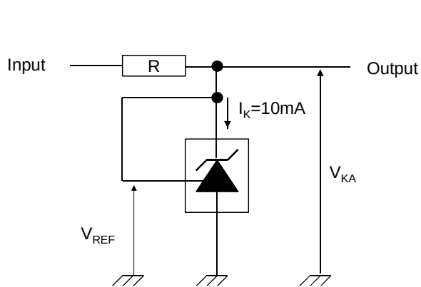
Figure 6. Test circuit V_{KA} = V_{REF}
