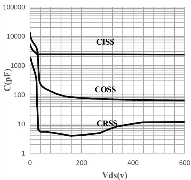
Figure 16: Typ. Capacitances
