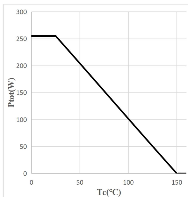
Figure 3: Power Dissipation
