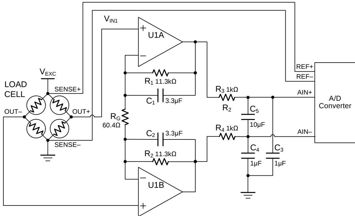
Figure12. Precision Weight Scale Measurement System
