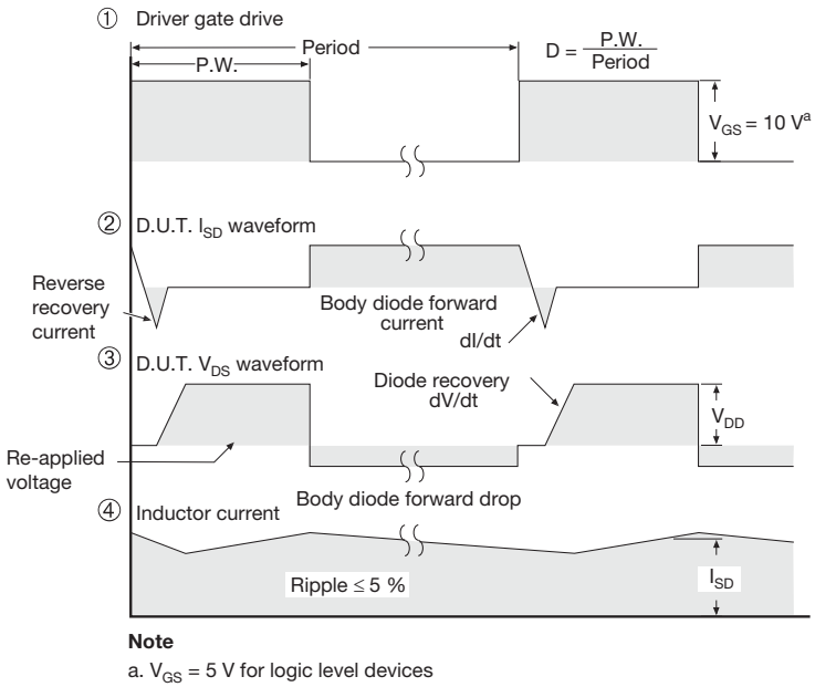
Fig. 18 - For N-Channel
