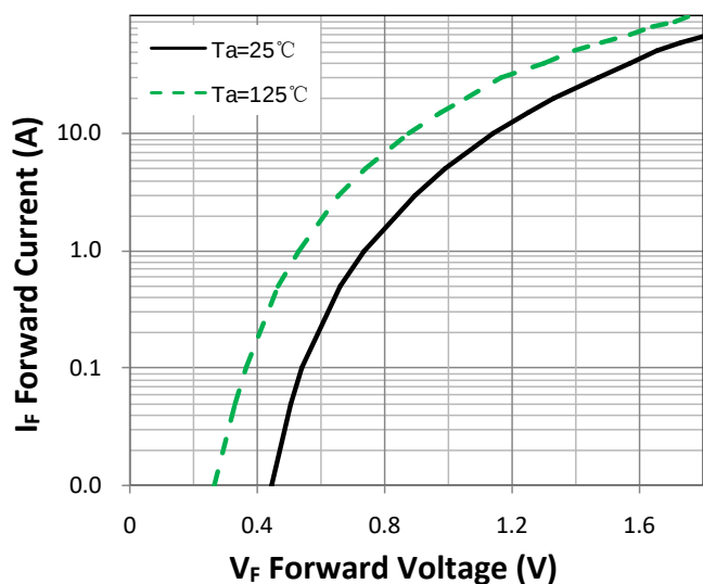
Figure 1. Forward Characteristic(typ.)
