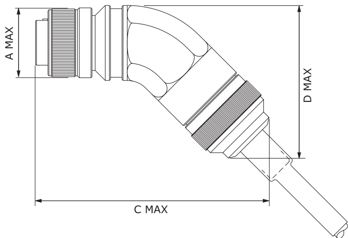
M28876/8 Plug with 45° Backshell
