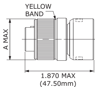
M28876/6 Plug
