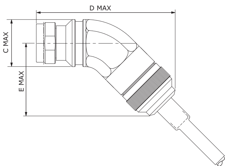
M28876/28 45° Backshell
