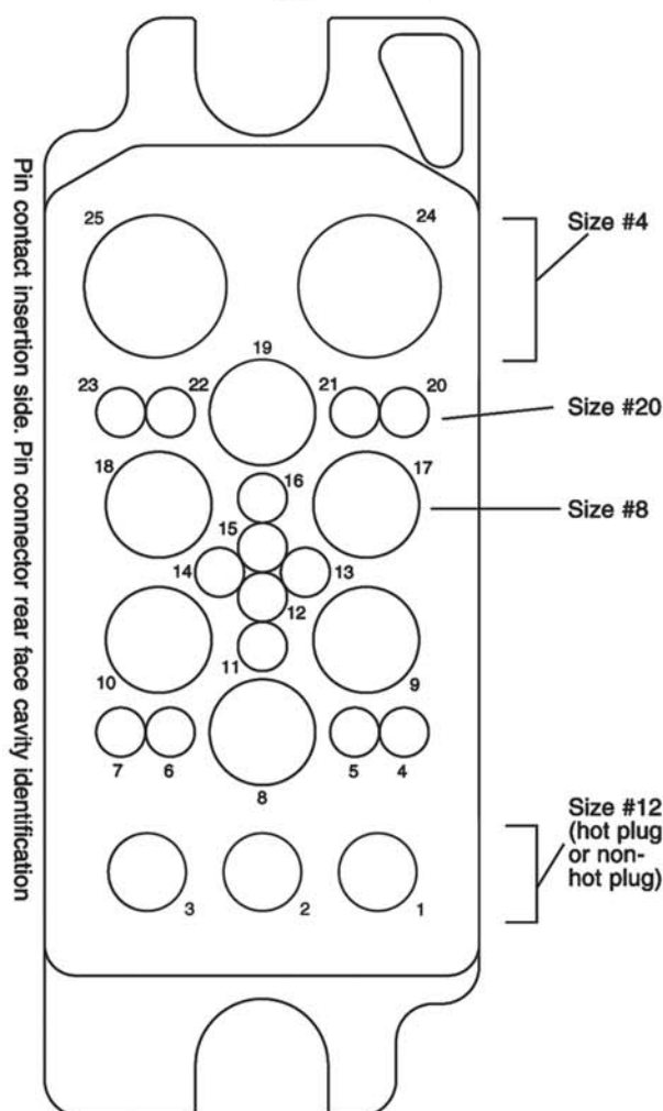
Pin housing (rear face)
