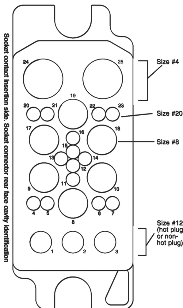
Socket housing (rear face)
