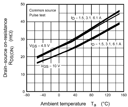
Fig. 8.2.6 R_{DS(ON)} - T_a
